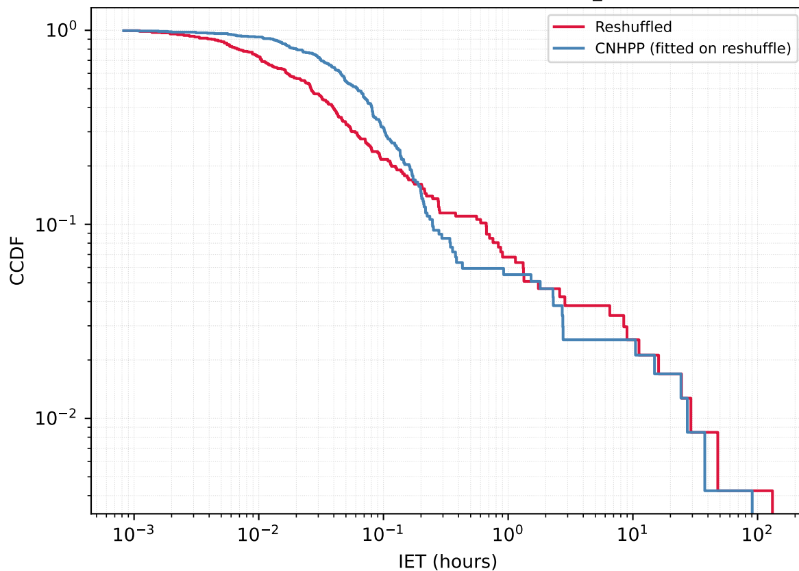
User 1095473116 - Reshuffled vs CNHPP A_{\text{fit}}=0.8074
